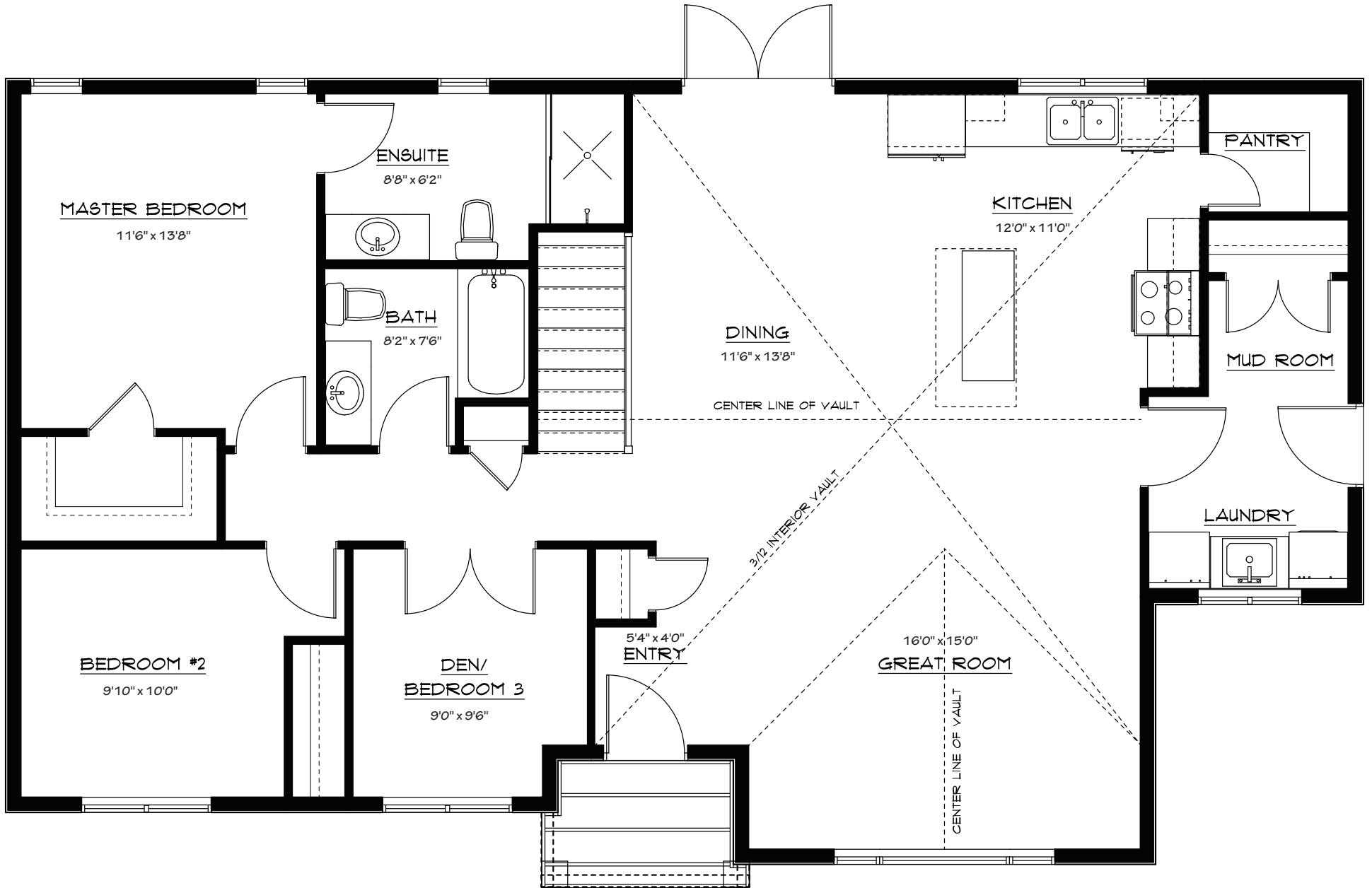
MAIN FLOOR LAYOUT THE RIVERSTONE 1,637 SQ. FT.
